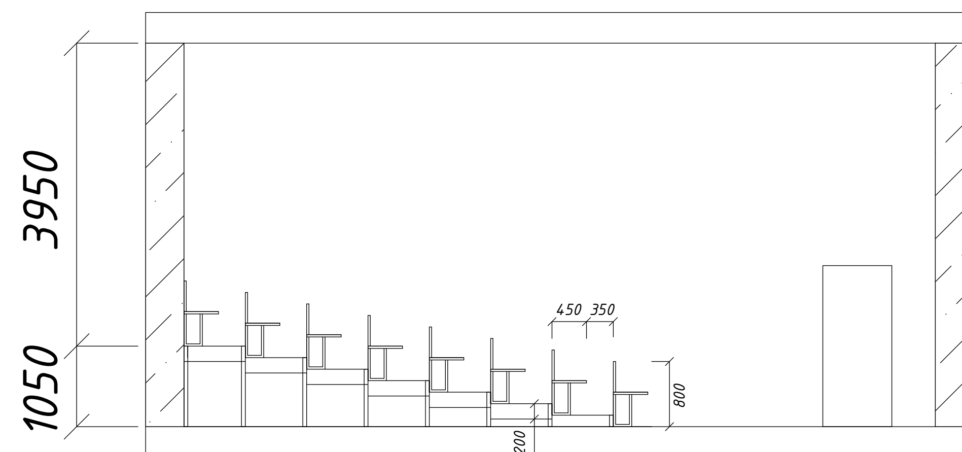
1-1 Lecture hall cross section
