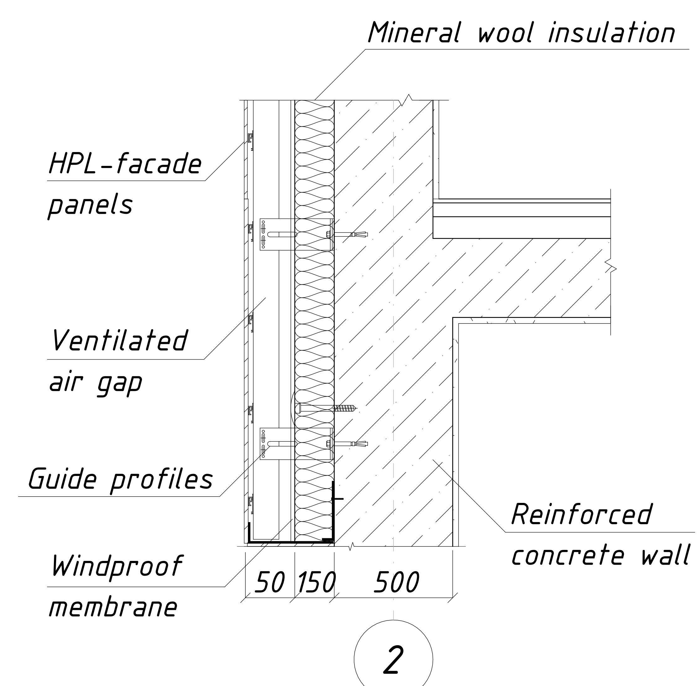
Ventilated facade system
