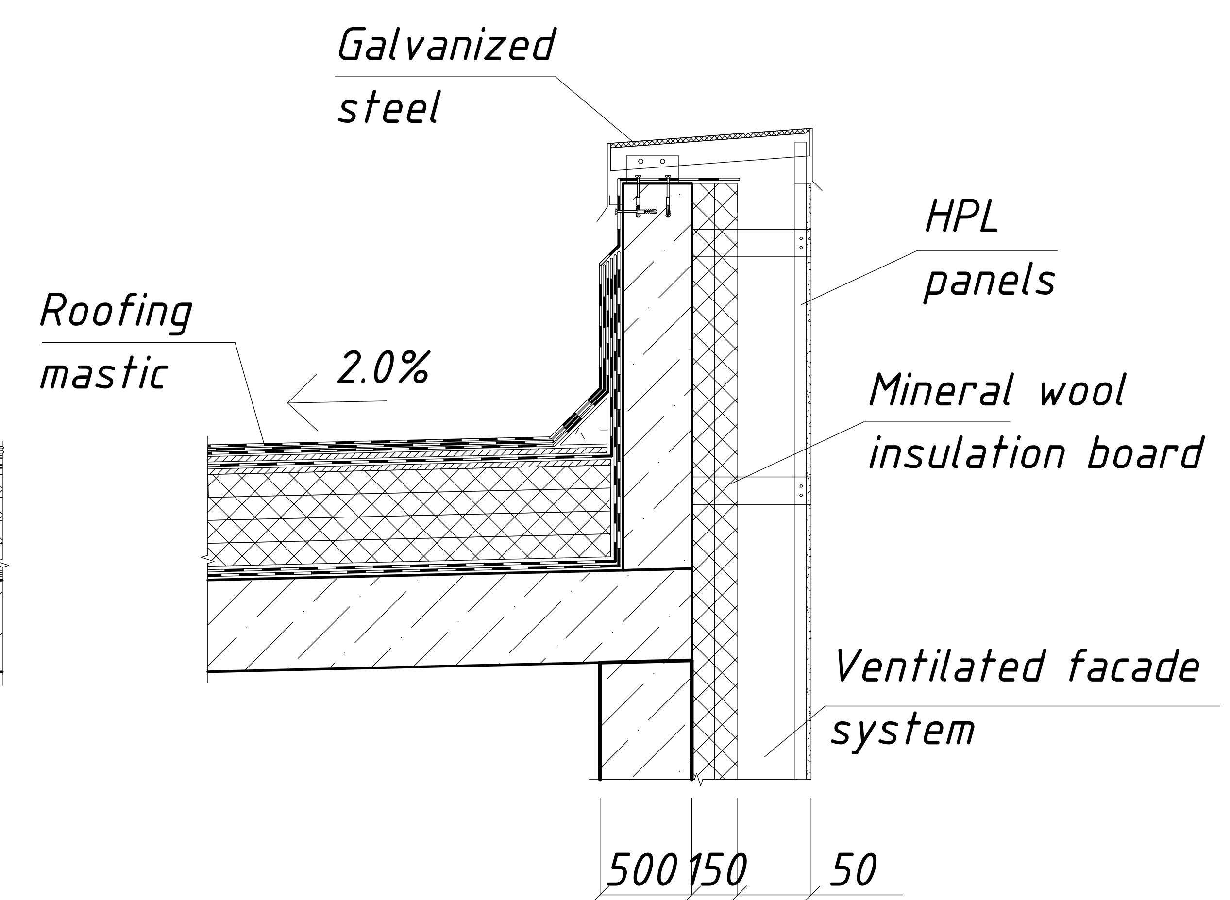
B Parapet detail
