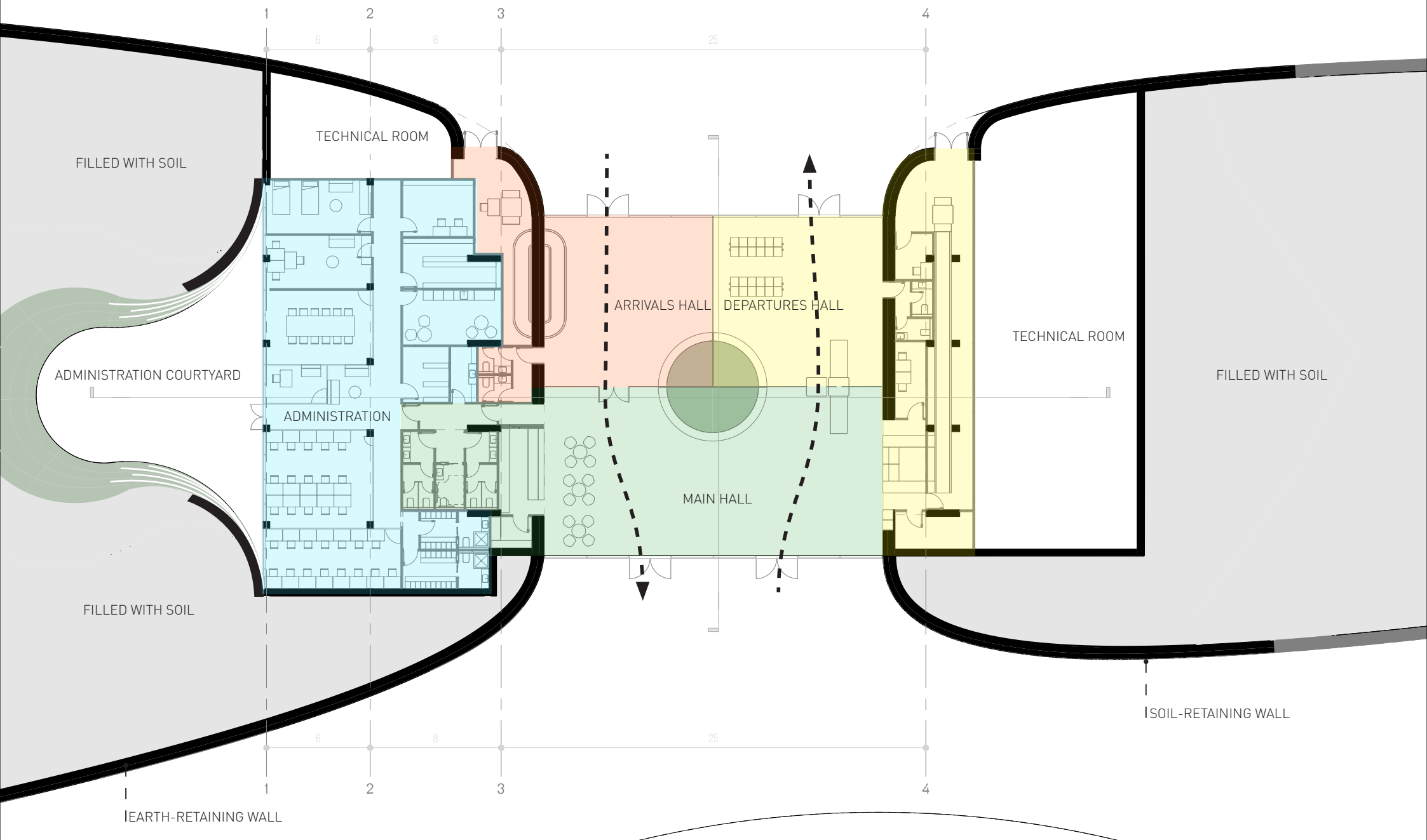
PLAN
