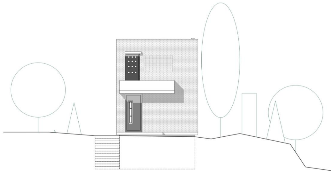
0 1 2 3m SOUTH-EAST ELEVATION
