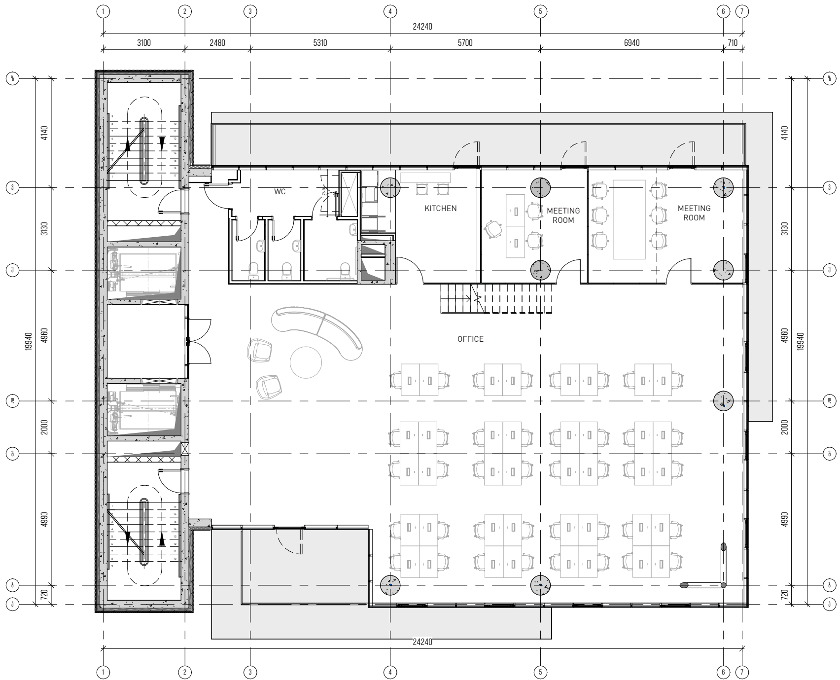
TYPICAL OFFICE PLAN
