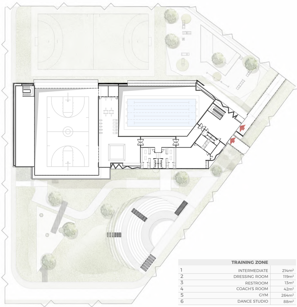
First Floor
