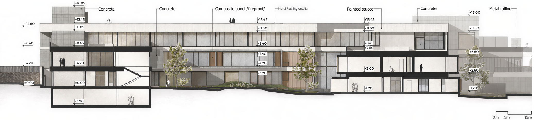
Section 4-4
